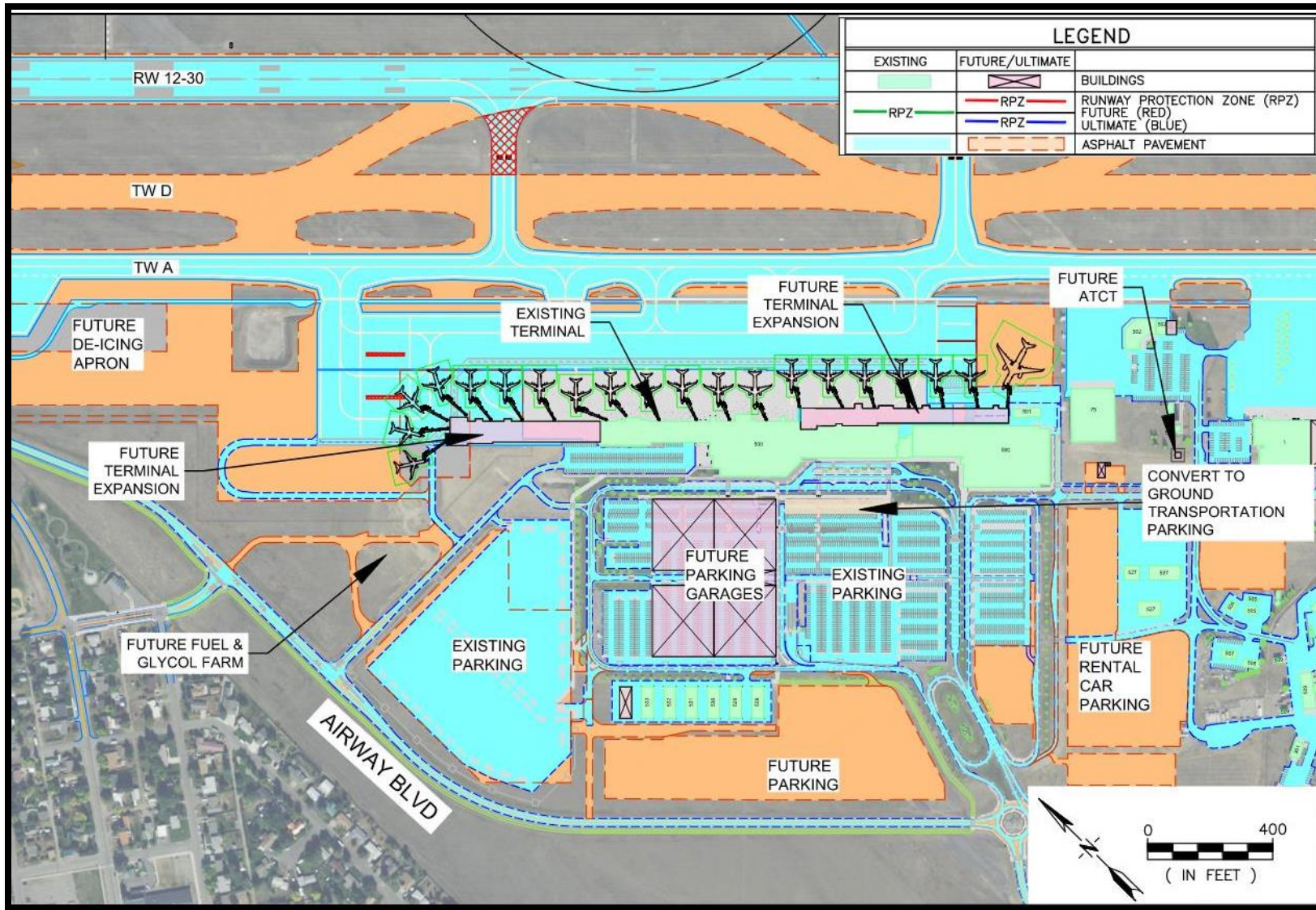
Figure 5-2: Recommended Alternative Passenger Terminal Complex
