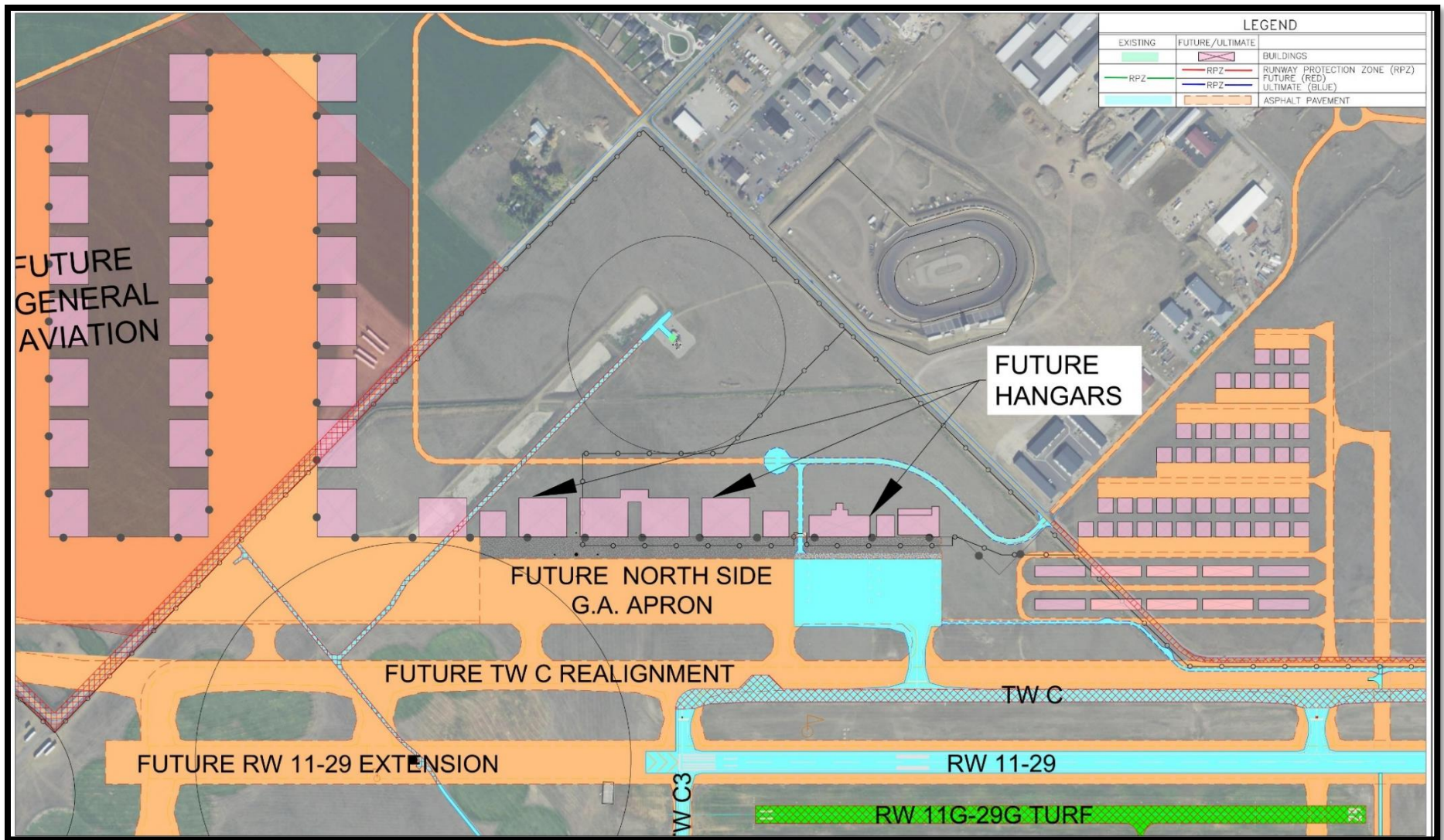
Figure 5-5: Recommended Alternative North General Aviation Area
